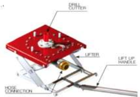
Mobile electric vehicle fire extinguishing device.
